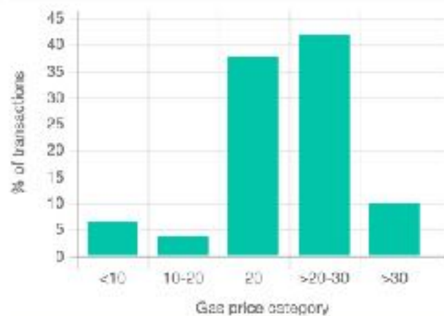
Transaction Count by Gas Price
