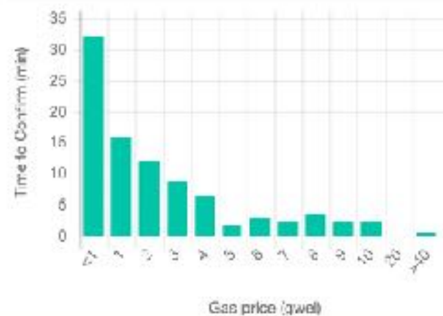
Confirmation Time by Gas Price
